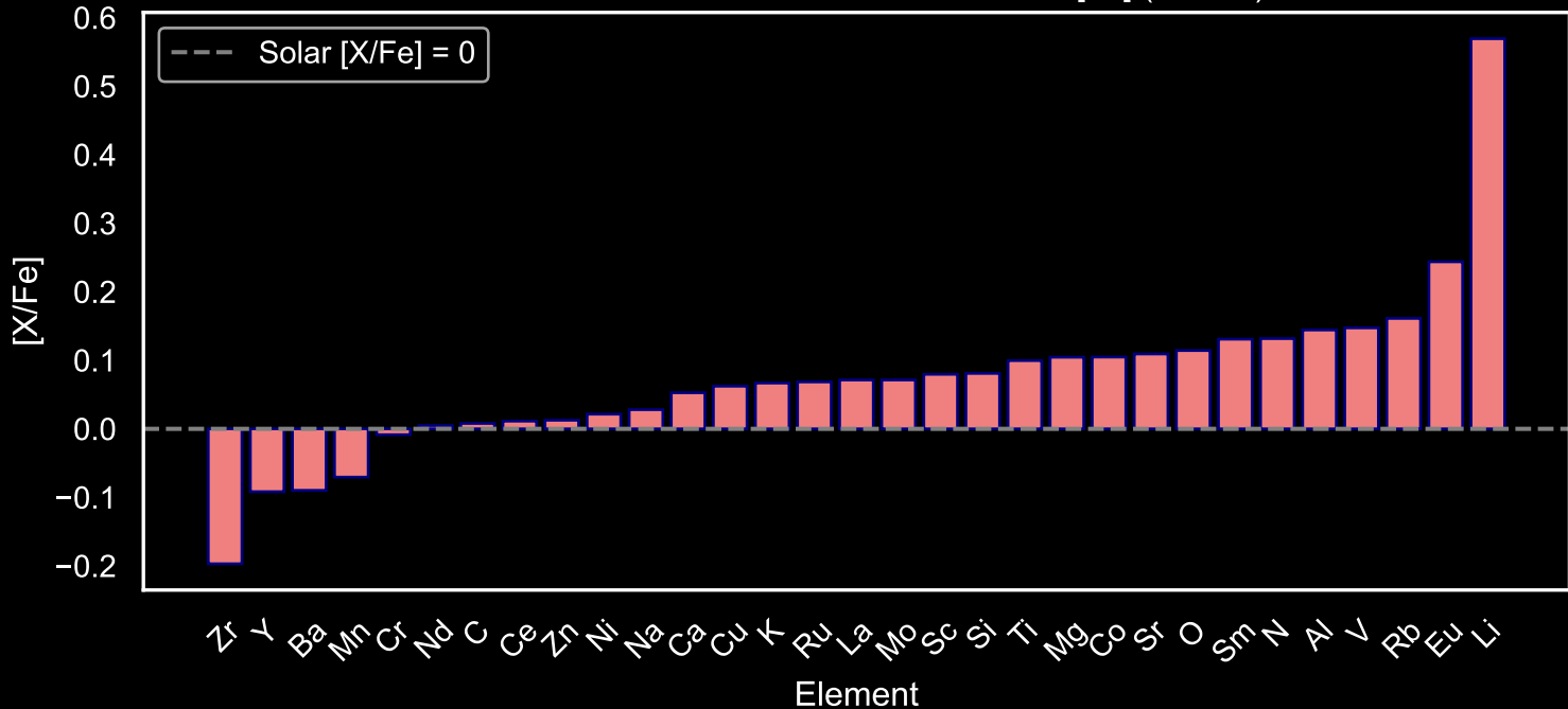
Abundance Pattern for GALAH Star Field [14] (N=315)
