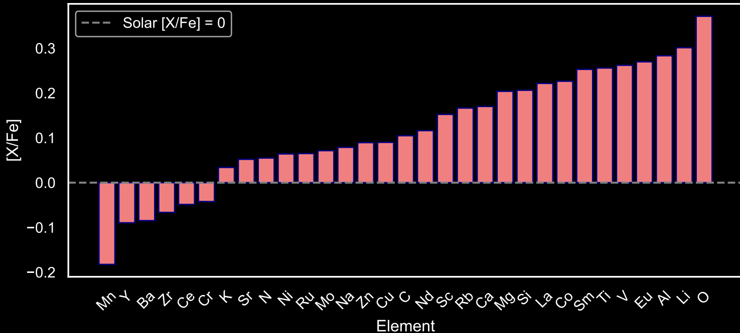
Abundance Pattern for GALAH Red Giants: Star Field [14] (N=65)
