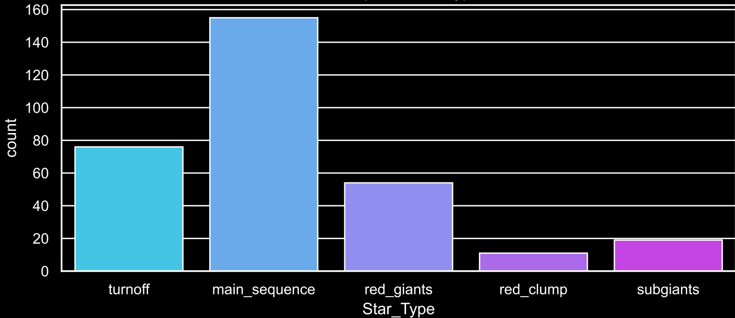
Field [14] Count plot of Star Type
