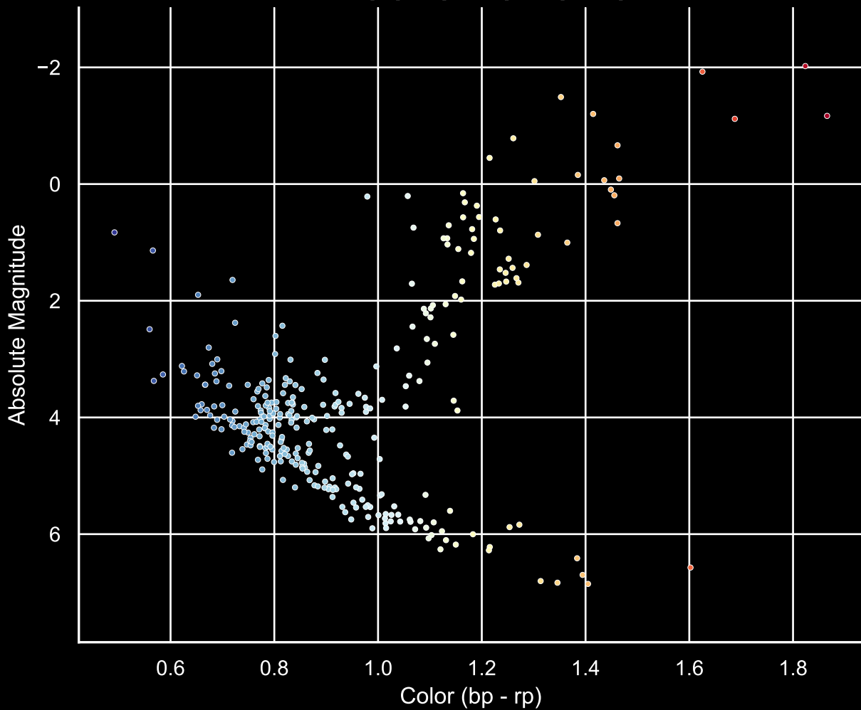
GALAH Hertzprung-Russel Diagram Field [14] Ra [324.86] Dec [-49.08]
