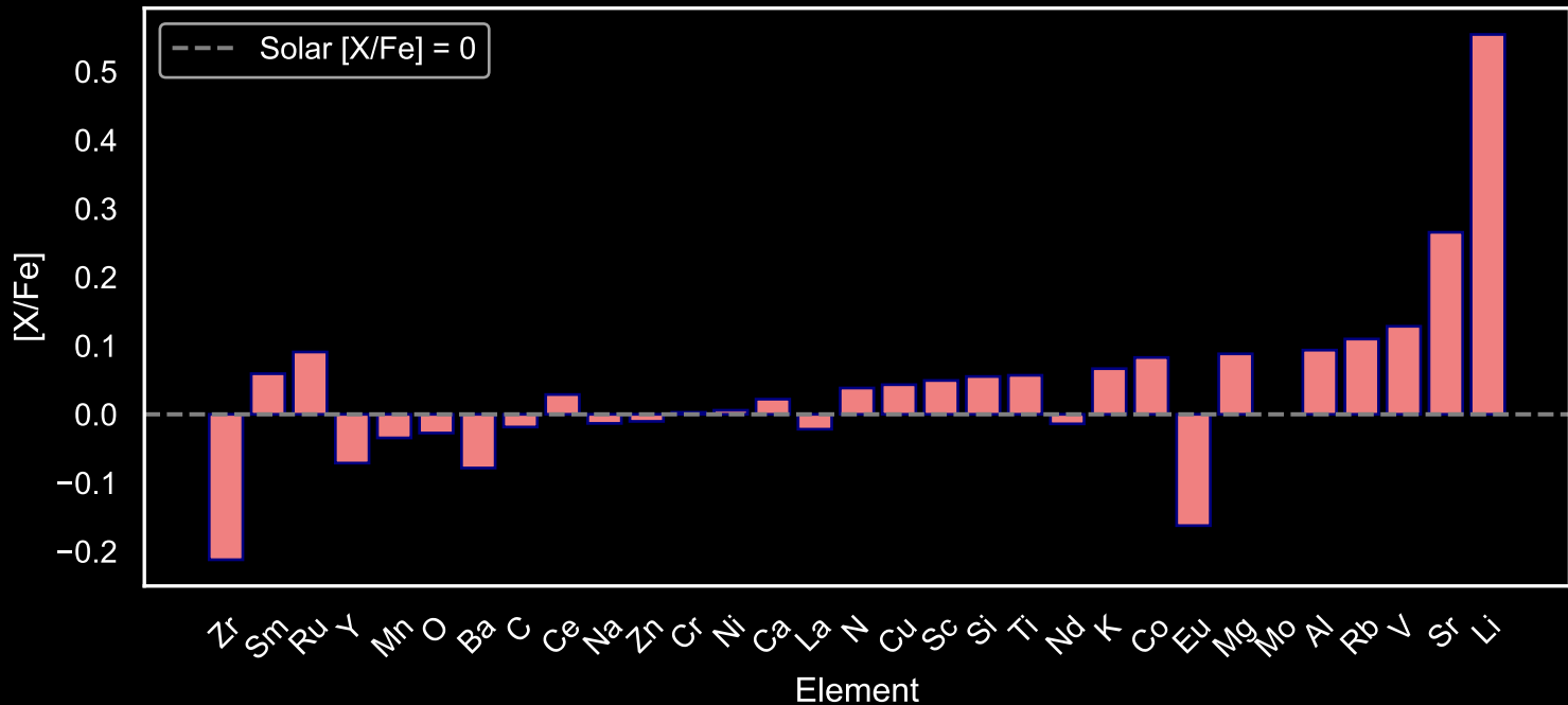
Abundance Pattern for GALAH Main Sequence Stars: Star Field [14] (N=155)
